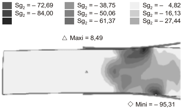
Figure 6. Distribution of stresses \sigma_y within the roll gap, with h_0 = 105,76 mm, \epsilon = 10\% , \theta = 4^\circ
