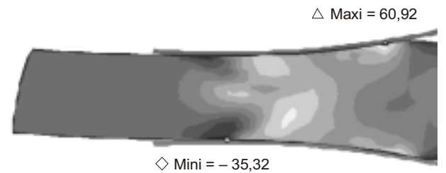
Figure 13. Distribution of stresses \sigma_m within the roll gap, with h_0 = 105,76 mm, \epsilon = 27,5\% , \theta = 4^\circ , positive values mean compression
