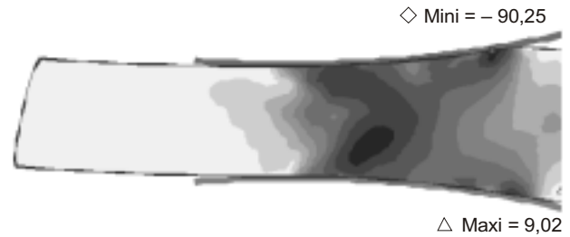
Figure 12. Distribution of stresses \sigma_y within the roll gap, with h_0 = 105,76 mm, \epsilon = 27,5\% , \theta = 4^\circ
