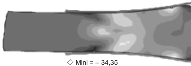
Figure 11. Distribution of stresses \sigma_m within the roll gap, with h_0 = 105,76 mm, \epsilon = 27,5\% , \theta = 2^\circ , positive values mean compression
