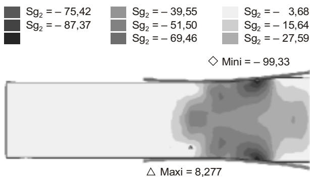
Figure 2. Distribution of stresses \sigma_y within the roll gap, with h_0 = 105,76 mm, \epsilon = 10\% , \theta = 0^\circ
