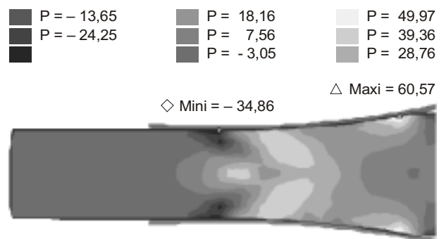
Figure 9. Distribution of stresses \sigma_m within the roll gap, with h_0 = 105,76 mm, \epsilon = 27,5\% , \theta = 0^\circ , positive values mean compression
