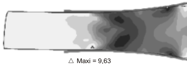
Figure 10. Distribution of stresses \sigma_y within the roll gap, with h_0 = 105,76 mm, \epsilon = 27,5\% , \theta = 2^\circ
