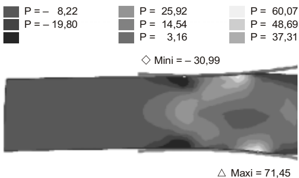
Figure 7. Distribution of stresses \sigma_m within the roll gap, with h_0 = 105,76 mm, \epsilon = 10\% , \theta = 4^\circ , positive values mean compression
