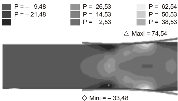
Figure 3. Distribution of stresses \sigma_m within the roll gap, with h_0 = 105,76 mm, \epsilon = 10\% , \theta = 0^\circ , positive values mean compression
