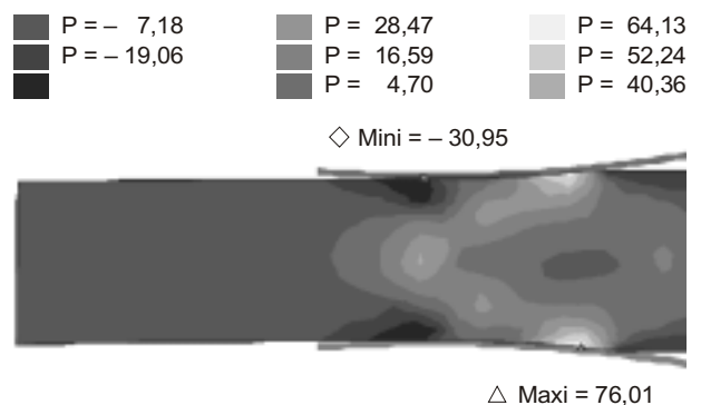
Figure 5. Distribution of stresses \sigma_m within the roll gap, with h_0 = 105,76 mm, \epsilon = 10\% , \theta = 2^\circ , positive values mean compression
