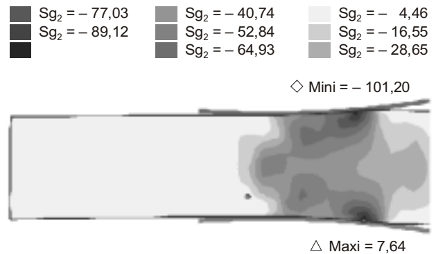
Figure 4. Distribution of stresses \sigma_y within the roll gap, with h_0 = 105,76 mm, \epsilon = 10\% , \theta = 2^\circ
