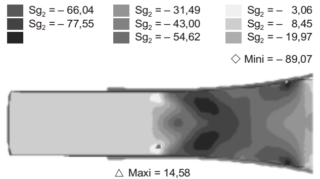
Figure 8. Distribution of stresses \sigma_y within the roll gap, with h_0 = 105,76 mm, \epsilon = 27,5\% , \theta = 0^\circ
