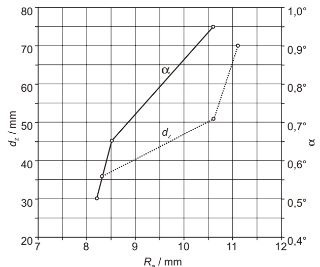
Figure 2. Influence of the grain diameter d_z and the impact angle \alpha of the blasting medium on the roughness R_a of the tested sheet at the air pressure p = 0,5 MPa
