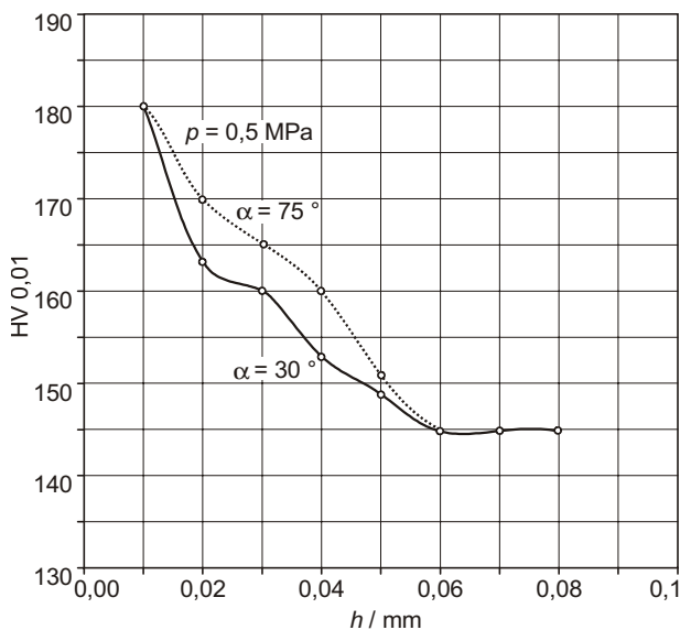
Figure 3. Course of the micro-hardness HV = 0,01 from the specimen surface h at various impact angles of the blasting medium
