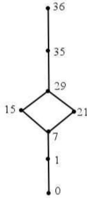
FIGURE 2. Submodule lattice of the 36 dimensional permutation module
