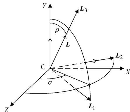
Figure 1 The coordinate system connected with vector \vec{L}
