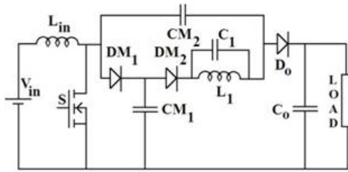
Fig. 1: Proposed converter circuit
