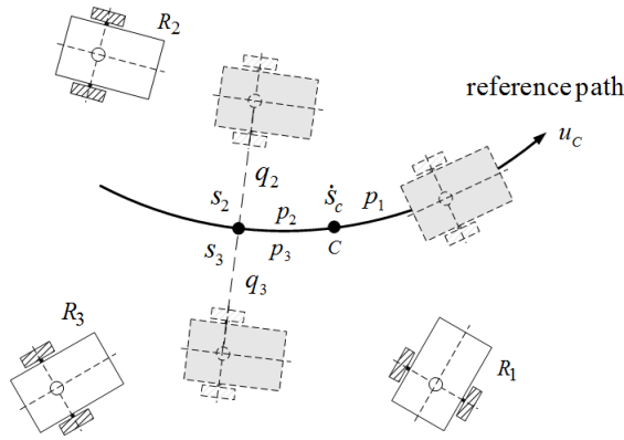
Fig. 1. Graphical depiction of mobile robots making a formation and following a reference path with offset quantities. Point C denotes the location of a virtual leader robot and $R_1 - R_3$ denote actual follower robots.
