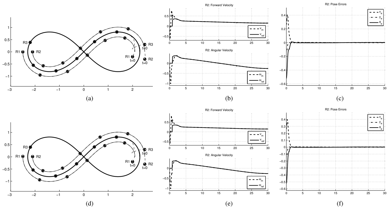
Fig. 5. The path following results by using two different values of the control horizon: (a) T_c = 0.25 s (i.e., 5 steps of the control horizon), (b) the velocity profiles of robot R_2 corresponding to (a), (c) the pose errors of robot R_2 corresponding to (a), (d) T_c = 0.5 s (i.e., 10 steps of the control horizon), (e) the velocity profiles of robot R_2 corresponding to (d), and (f) the pose errors of robot R_2 corresponding to (d).
