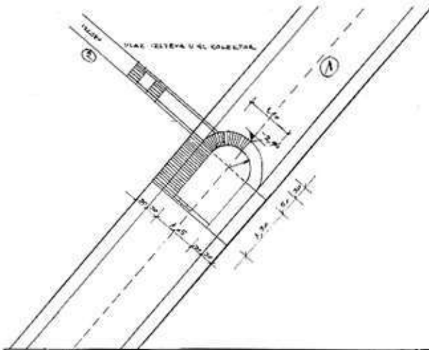
Sl. 9 Nalaz rimskog kolektora u Kranjčevićevoj ulici prilikom gradnje stambene zgrade »Rafinerije« Find of the Roman main sewer in Kranjčevićeva street during the construction of the residential building of »Rafincija«
