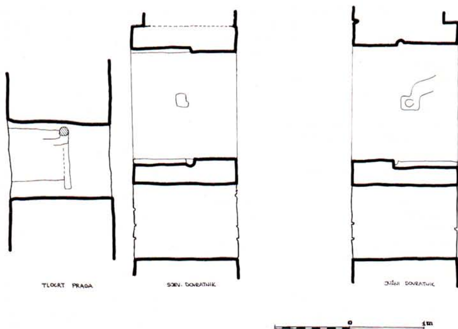
11 Detalj praga i dovratnika u mauzoleju (A. F.) Details of the mausoleum door-step and threshold.
