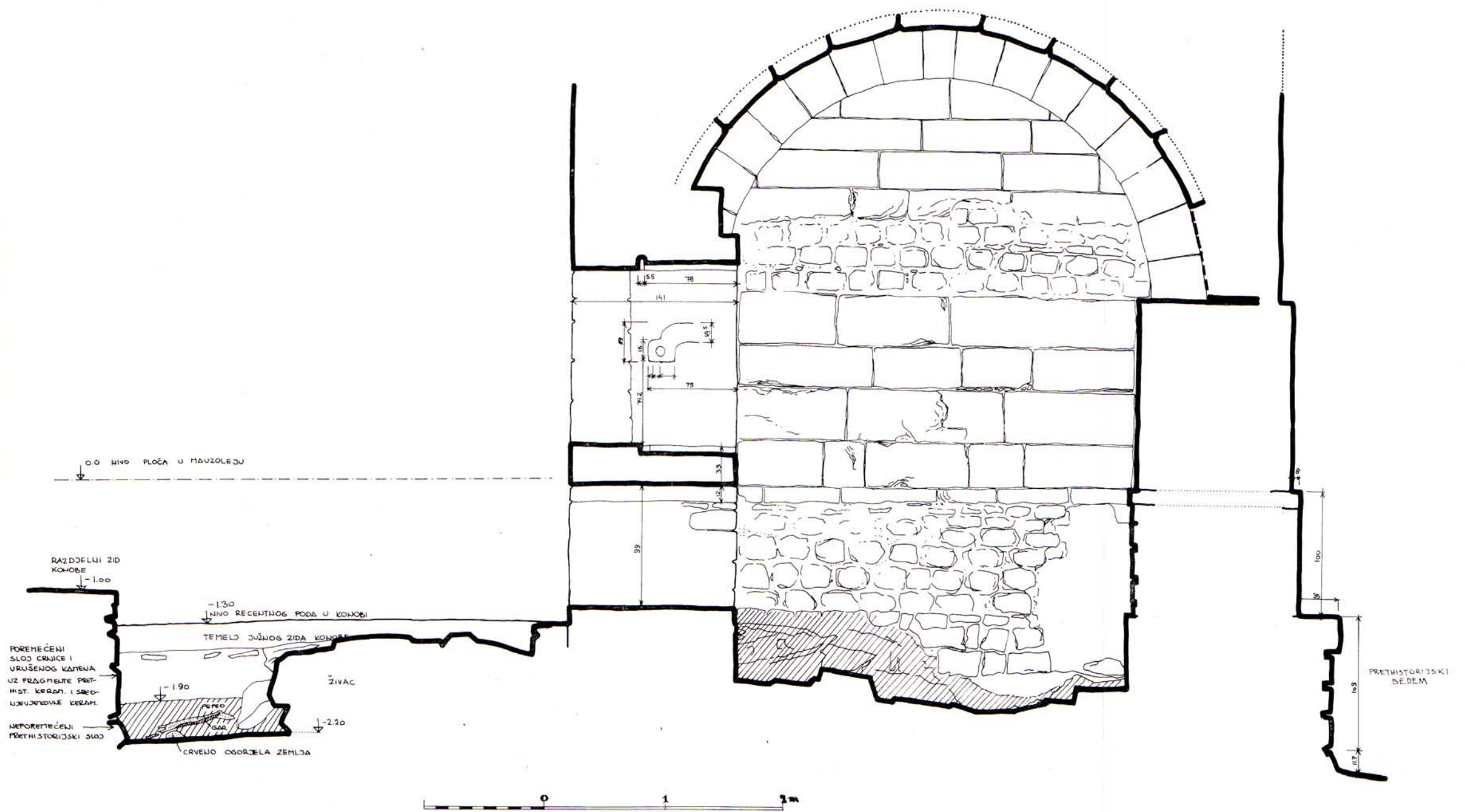
9. Presjek I—Z kroz vrata mauzoleja (A. Faber-S. Machiedo) E—W section through the mausoleum door.
