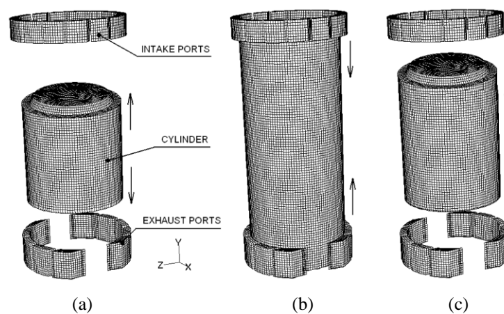
Fig. 3 Mesh motion. (a) 90^\circ lower crankshaft angle; (b) 200^\circ lower crankshaft angle; (c) 270^\circ lower crankshaft angle
