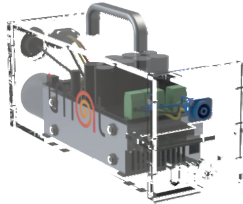
Figure 14. The IMAT Power Box, rendered here, is subdivided in its main components: the IMAT Main Board and the AC/DC Switching Power Supply, which assures galvanic insulation of the output voltage
