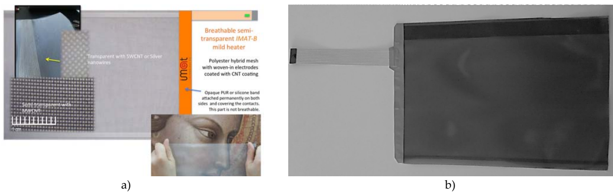
Figure 9. a) Conceptual design of IMAT breathable semi-transparent heater; b) standard textile-based heater coated with Carbo-e-Therm
