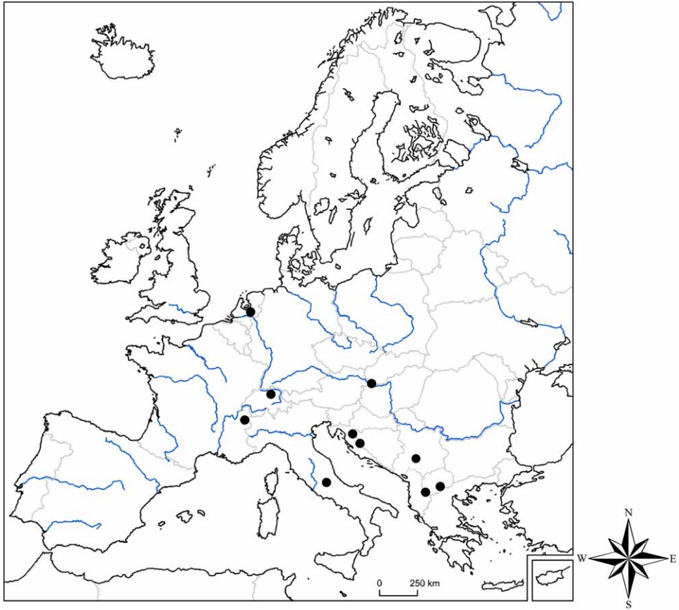
On-line Supplement Fig. 1. European distribution of Navicula jakovljevicii .
