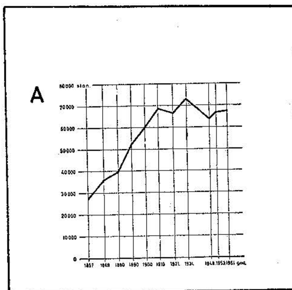
Fig. 3. A) Population changes in the Daruvar-Pakrac area from 1857 to 1961.
