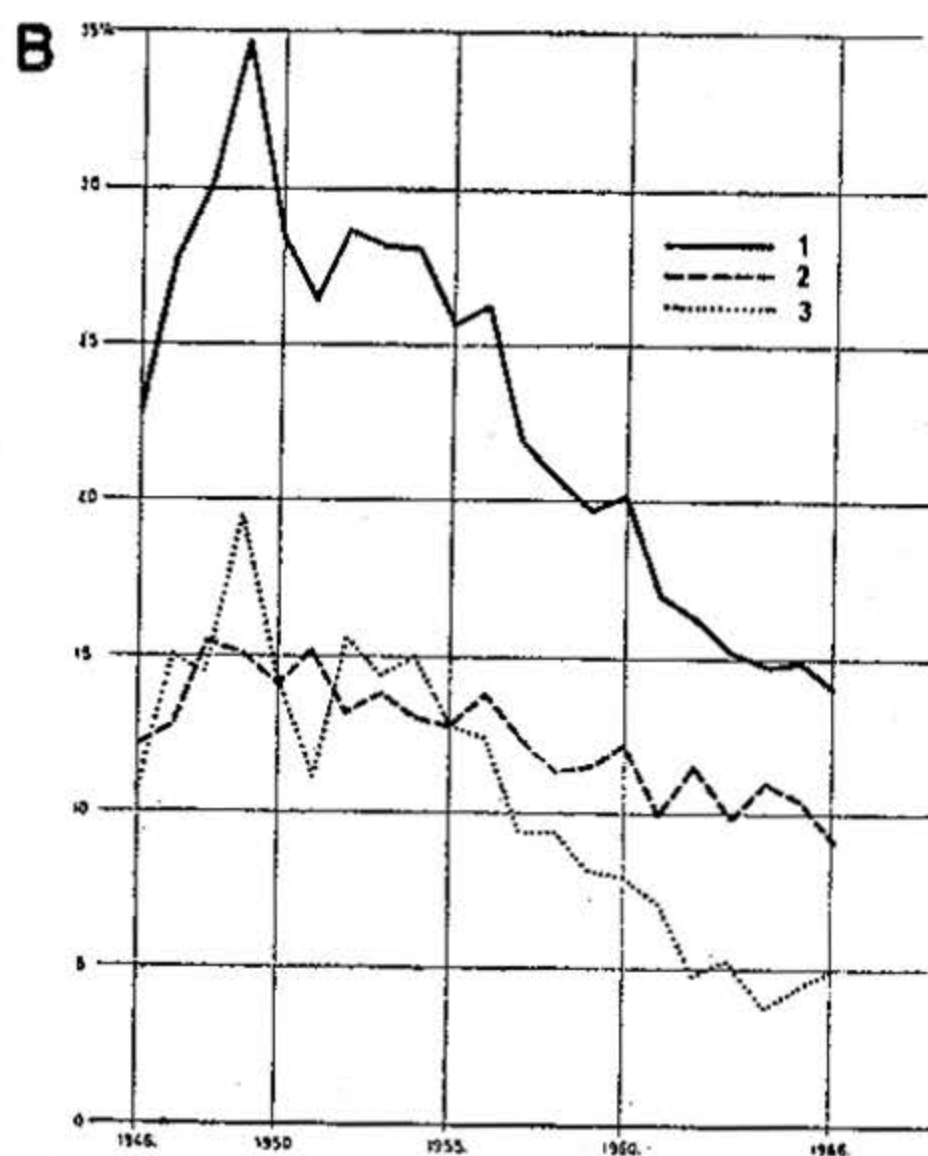
Fig. 3, B) Changes of the relative value of birth rate, death rate, and natural increase in the Daruvar-Pakrac area from 1946 to 1967. 1 — natality, 2 — mortality, 3 — natural increase
