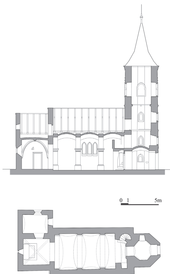
10. Župna crkva svete Ane u Beletincu, aktualno stanje. Nacrt prema: [Vukičević-Samaržija - 1993.], str. 149 / Parish church of St. Anne at Beletinec, current state. Plan according to: [Vukičević-Samaržija - 1993.], p. 149
