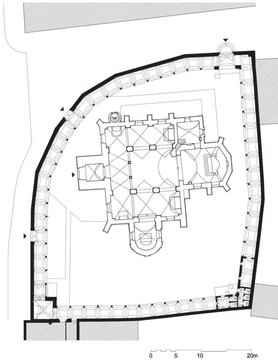
3. Tlocrt cinktora i župne crkve – postojeće stanje (Vedran Linke, d. i. a, Blanda Matica, d. i. a., planoteka IPU) / Ground-floor plan of the Ludbreg church and arcaded porch – present condition (by Vedran Linke, Blanda Matica, Plan Collection of the Institute of Art History)
