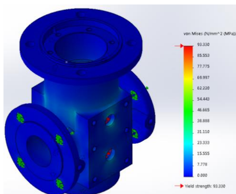
Figure 18. Results of the stress analysis of the housing of the three-spindle screw pump with the test pressure 1,5 MPa (15 bars), wall thickness \delta = 6,5\text{ mm} and material NL – 42
