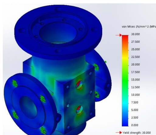
Figure 20. Results of the stress analysis of the housing of the three-spindle screw pump with the test pressure 1,5 MPa (15 bars), wall thickness \delta = 8,5\text{ mm} and material AlSiMg
