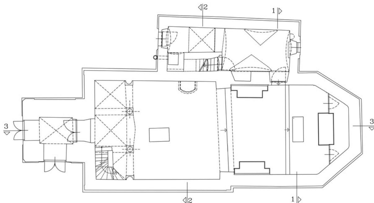
4. Kapela sv. Lovre, tlocrt prizemlja (planoteka KO u Varaždinu, izradila B. Petanjek) Chapel of St. Lawrence, ground view (Plan Archive of the Conservation Department in Varaždin, drawing by B. Petanjek)
