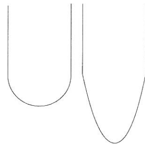
Fig. 1. Left: A connection of two straight lines minimizing the first derivative of \mathbf{v}(s) . Right: A connection of two straight lines minimizing the second derivative of \mathbf{v}(s) (like a hanging rope).
