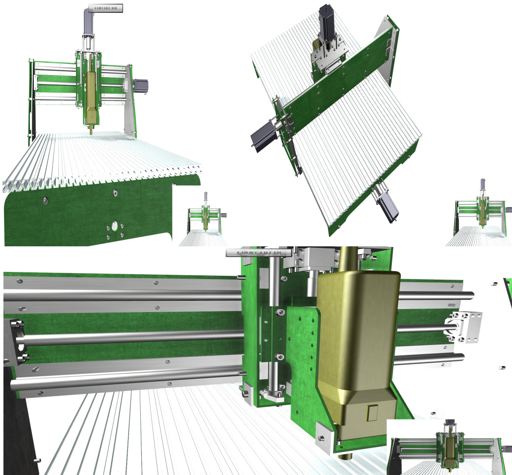
Fig. 25 Visualisation of whole CNC portal machine tool in EON studio software
