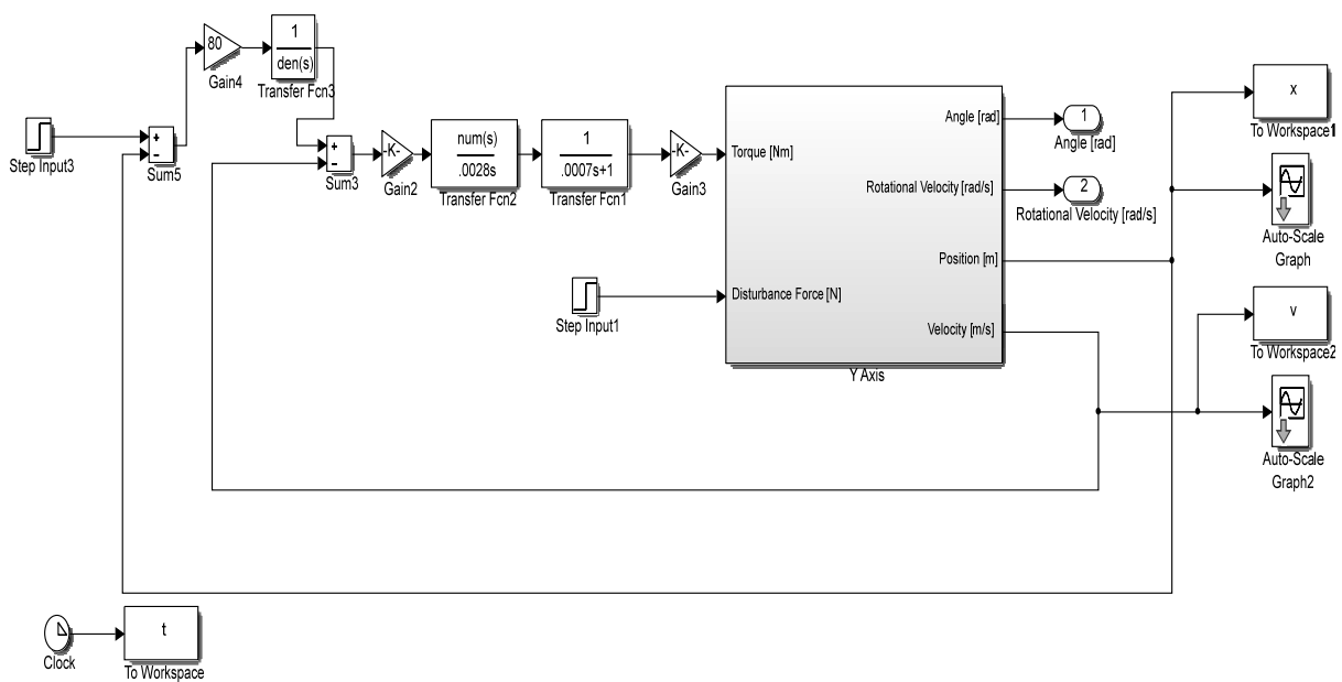
Fig.14 Multibody Sim Scape model of Y-axis feed drive of virtual CNC portal milling machine
