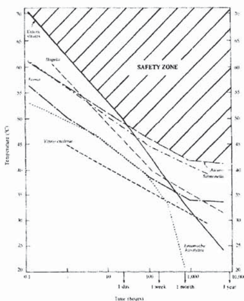
Figure 1. - TIME-TEMPERATURE REQUIREMENTS TO PRODUCE SLUDGE, THAT IS VIRTUALLY PATHOGEN-FREE. (Feachem, 1983)
