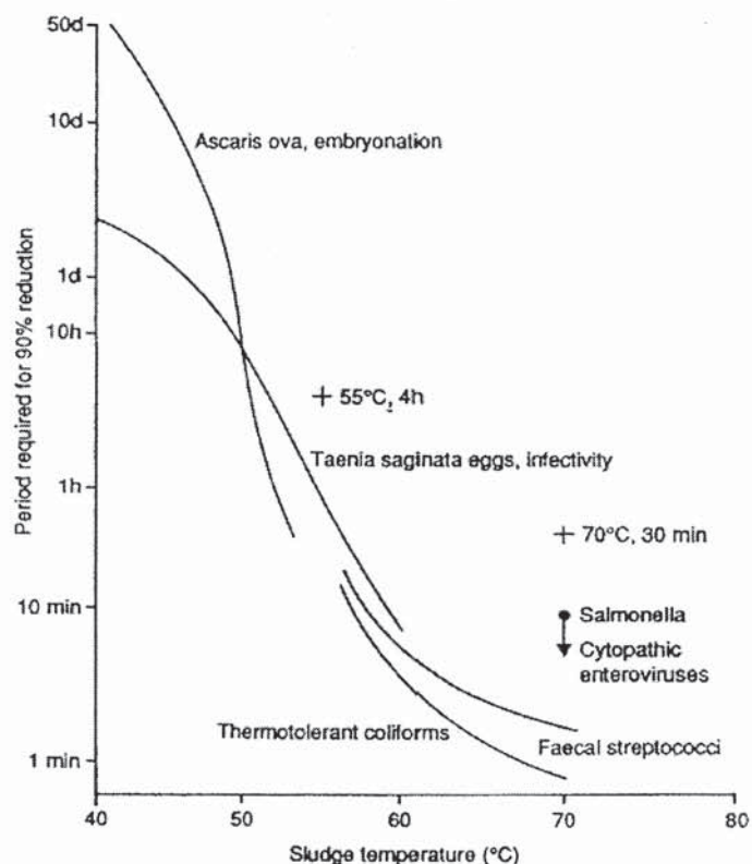
Figure 2. - EFFECT OF SLUDGE TREATMENT TEMPERATURE UPON TIME FOR 90% DESTRUCTION OF VARIOUS PATHOGENS. CROSSES INDICATE TEMPERATURE/TIME CONDITIONS SPECIFIED IN CODE OF PRACTICE (DoE, 1989) (Pike and Carrington, 1986).
