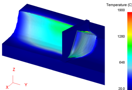
Fig. 3 Temperature field in the cutting zone
