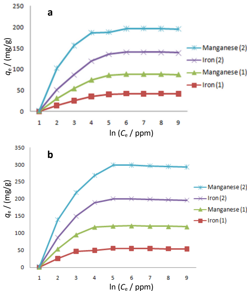
Figure 5. Temkin adsorption isotherms of manganese and iron ions: cellulose membrane (a) and composite membrane (b)
