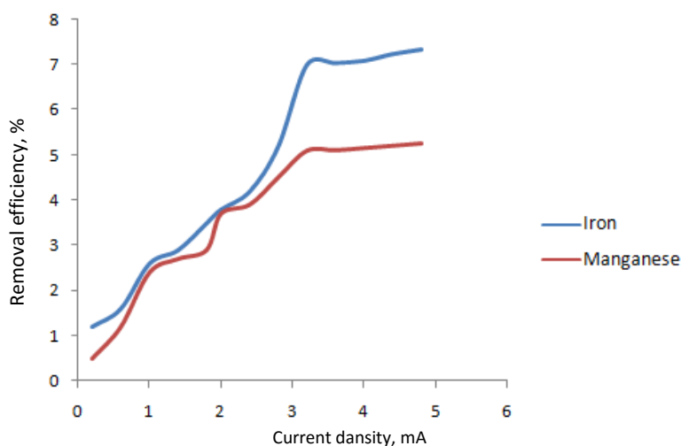
Figure 3. Effect of current density on iron and manganese removal.
