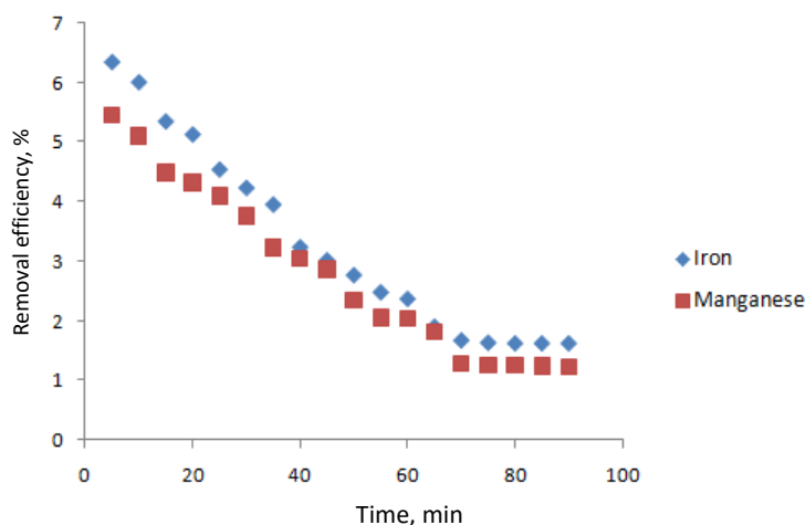
Figure 1. Iron and manganese concentration evolution in time in the case photo-electrochemical combined with electrocoagulation method
