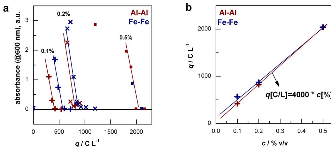
Figure 3. (a) Absorbance of the clear part of the liquid as function of charge passed between Al-Al electrodes (red symbols) and between Fe electrodes (blue symbols) for emolin-water emulsions of concentrations as indicated. (b) Charge needed for the effective coagulation.
