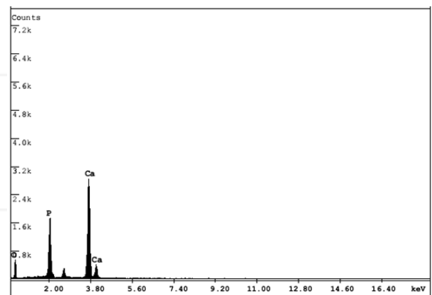
Figure 13. EDX spectrum of the HAp
