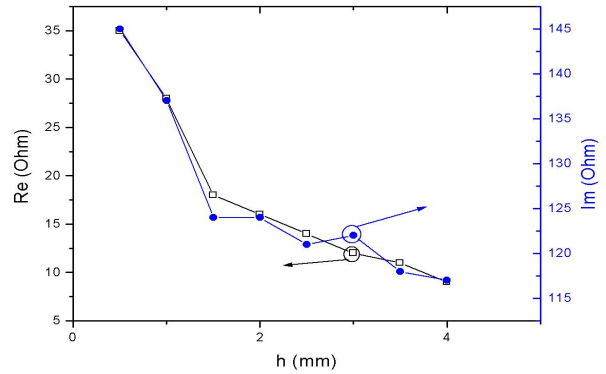
Figure 6. (d) Results of the analysis of influence of the loop distance h from the feed line on the antenna input impedance.
