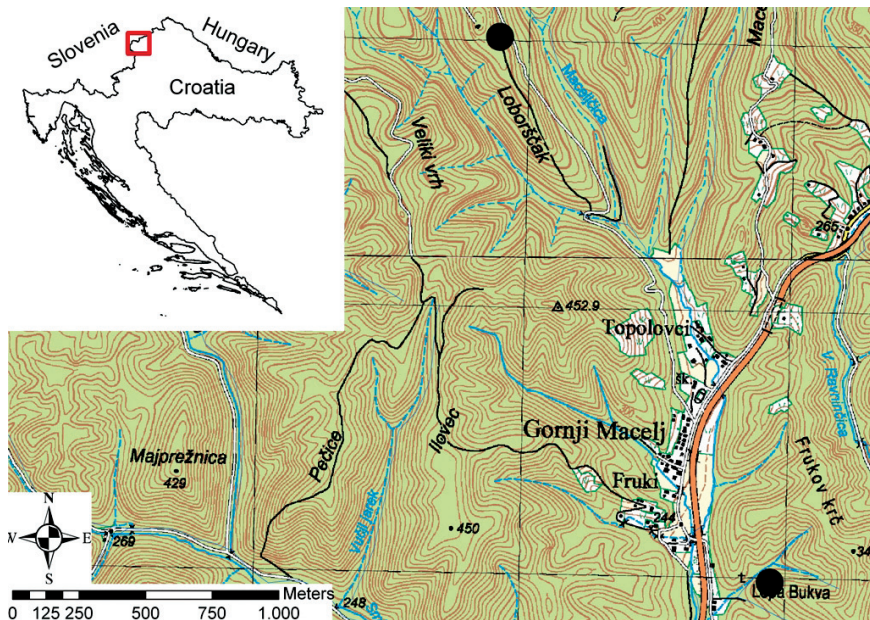
Fig. 1. Research area on Macelj Mountain, with black spots representing records of Zootoca vivipara .
