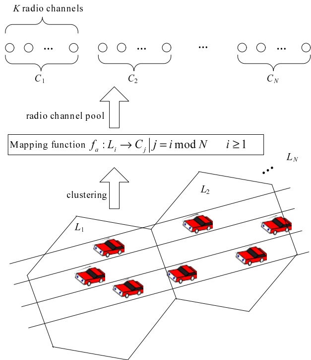
Fig. 1. The model of clustering based MAC Scheme.
