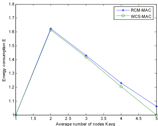
Fig. 6. Energy consumption comparison for different values of K_{avg}
