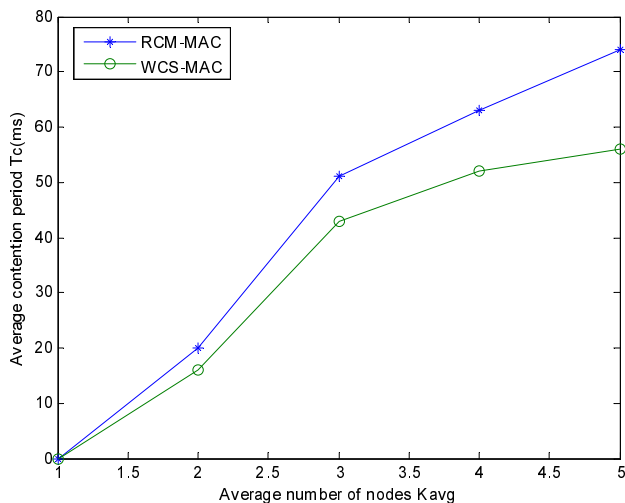
Fig. 7. Average contention period comparison for different values of K_{avg}
