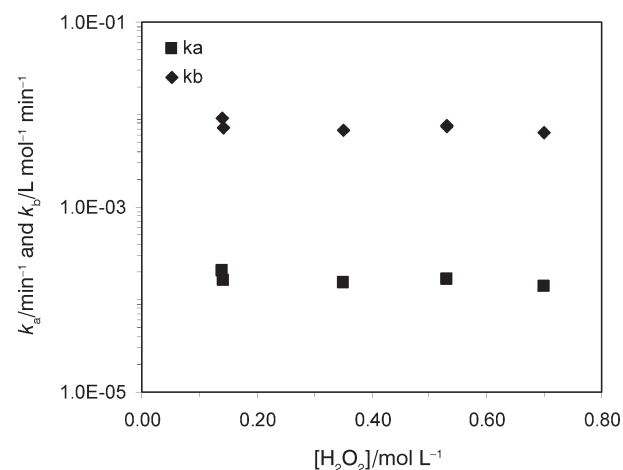
Fig. 3 – Effect of [\text{H}_2\text{O}_2] on rate coefficients k_a and k_b for the hydrogen peroxide decomposition in presence of pyrite grains ( A = 0.0121 \text{ m}^2 \text{ g}^{-1} ) at \text{pH} 1.00 and 25 \text{ }^\circ\text{C} temperature
