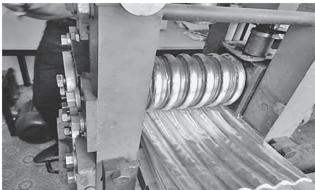
Figure 1 Duo rolling mill with the corrugated rolls
