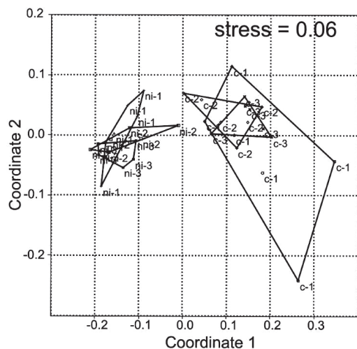
Figure 3. Diagram of non-metric multidimensional scaling (NMDS) performed on Bray-Curtis similarity matrix of ground beetle assemblages, ni- assemblages of non-inversion tillage, c- assemblages of conventional tillage
