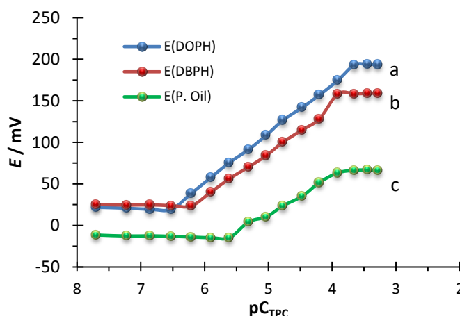
Figure 5. Optimization of plasticizers with CPE compositions: (a) DOP 46.5 %, graphite 46.5 %, IP 7.0 %, (b) DBP 46.0%, Graphite 46.0 %, IP 8.0 %), (c) p. Oil 45.0 %, graphite 45.0, IP 10.0 %.
