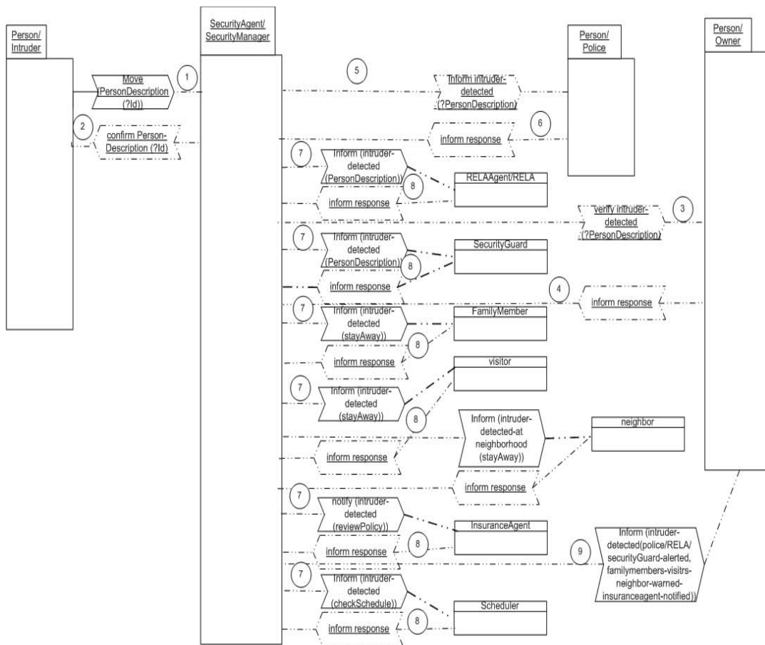
Figure 6. Interaction sequence diagram from intruder handling.
