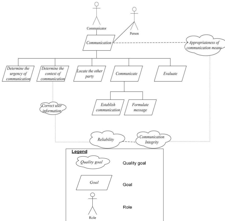
Figure 2. Goal model for communication.
