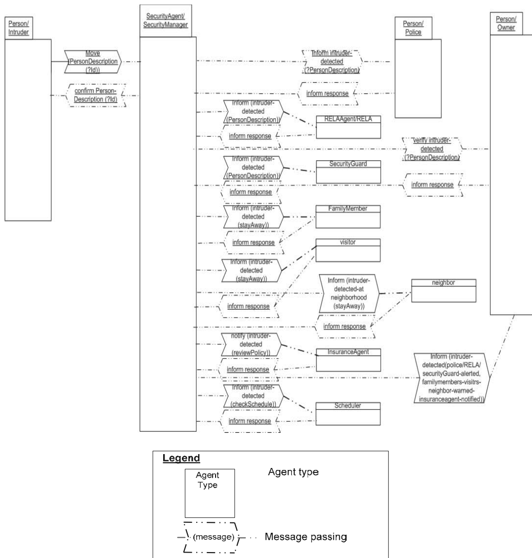
Figure 3. Interaction-frame diagram for intruder handling.
