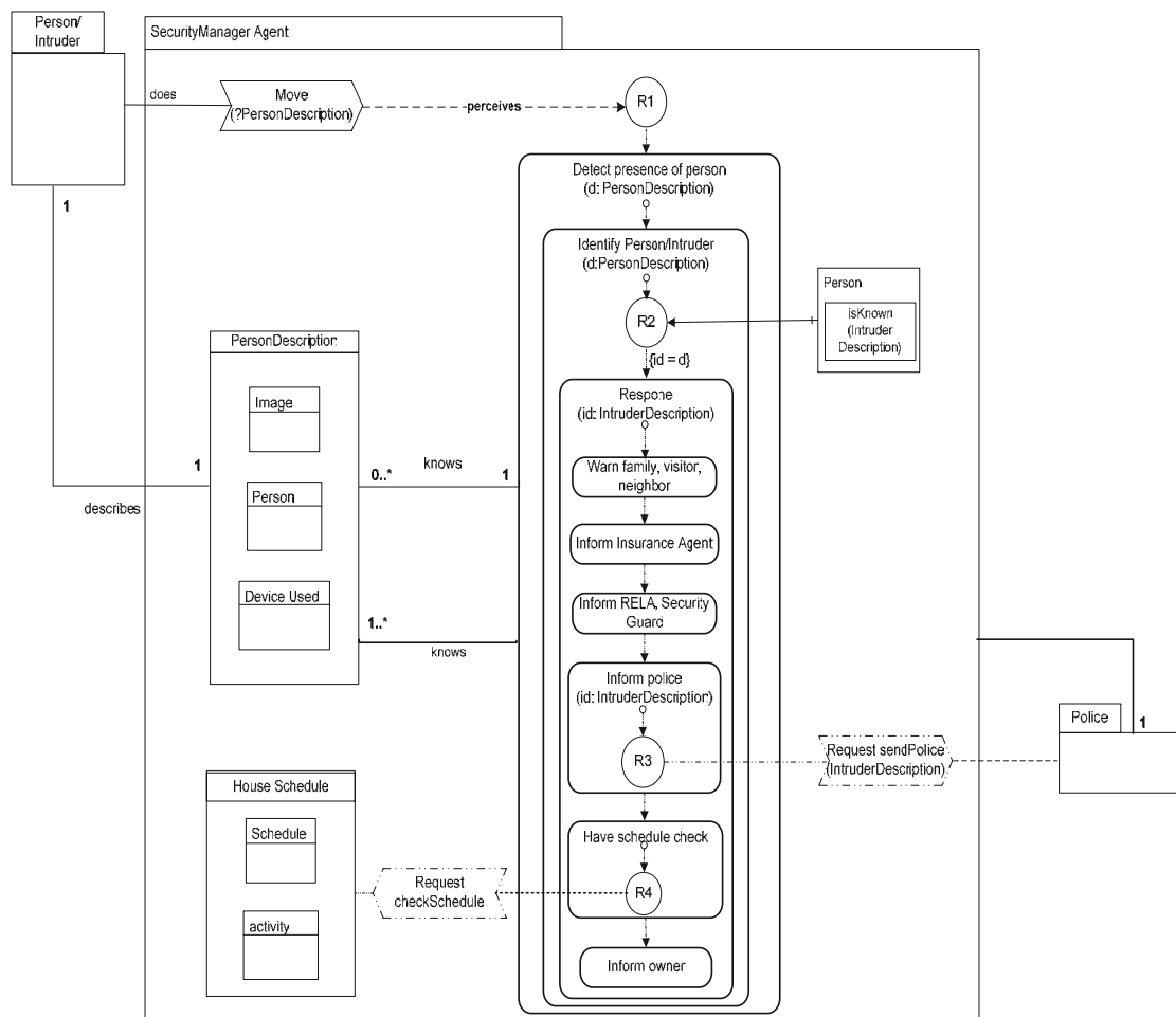
Figure 7. The behaviour model for the intruder-handling.
