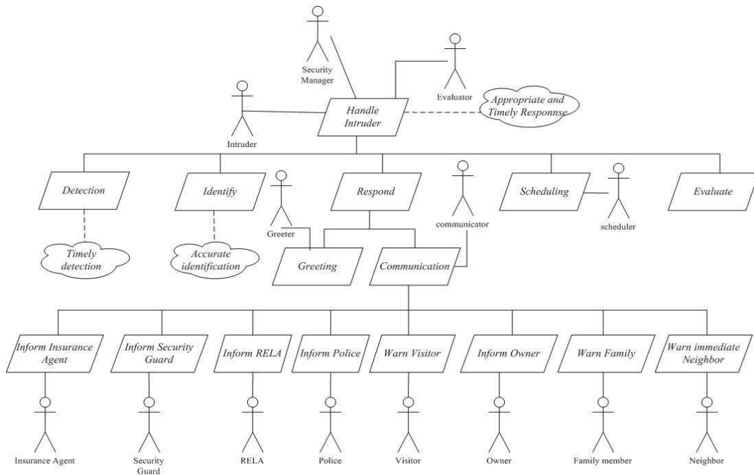
Figure 1. The goal model for intruder handling.
