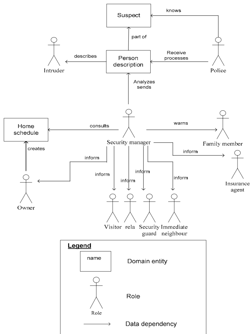
Figure 4. The domain model for intruder handling.
