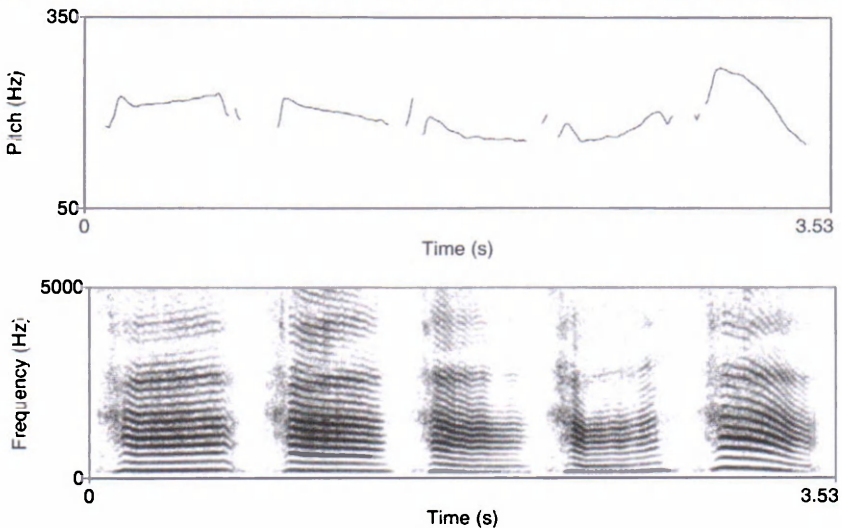
Slika 8c. Akustički prikaz pet tajskih tonema: k h á: (visoki) ‘trgovati’, k h ā: (srednji) ‘zaglaviti’, k l ā: (niski) ‘smeđi šećer’, k h ā: (uzlazni) ‘noga’, k h ā: (silazni) ‘ja’ Figure 8c. Acoustics of five Thai tones: k h ā: (high) ‘to engage in trade’, k h ā: (mid) ‘to get stuck’, k h ā: (low) ‘galangal’, k h ā: (rising) ‘leg’, k h ā: (falling) ‘I’
