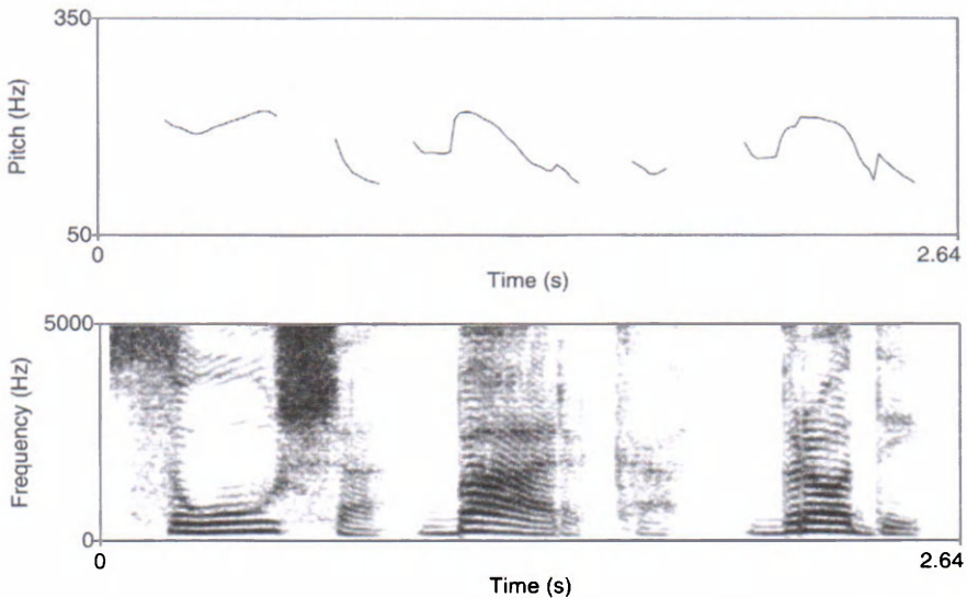
Slika 6b. Akustički prikaz hrvatskih čakavskih naglasaka (s naglašenim prvim slogom): sūša (akut), bārka (ds), brōdi (ks) Figure 6b. Acoustics of Croatian Čakavian pitch-accents (on the word initial syllable): sūša (acute) ‘drought’, bārka (LF) ‘boat’, brōdi (SF) ‘ships’
