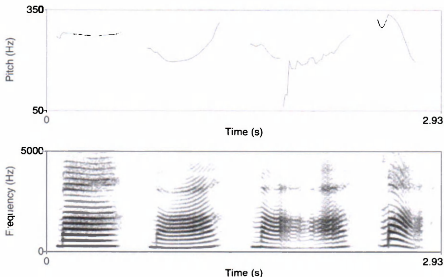
Slika 7b. Akustički prikaz četiriju kineskih tonema: mā (ton 1, ˩) 'majka', má (ton 2, ˨˨) 'konoplja', mǎ (ton 3, ˨˨˨) 'konj', mà (ton 4, ˨˨˨˨) 'grditi' Figure 7b. Acoustics of four Chinese tones: mā (ton 1, ˩) 'mother', má (ton 2, ˨˨) 'hemp', mǎ (ton 3, ˨˨˨) 'horse', mà (ton 4, ˨˨˨˨) 'scold'
