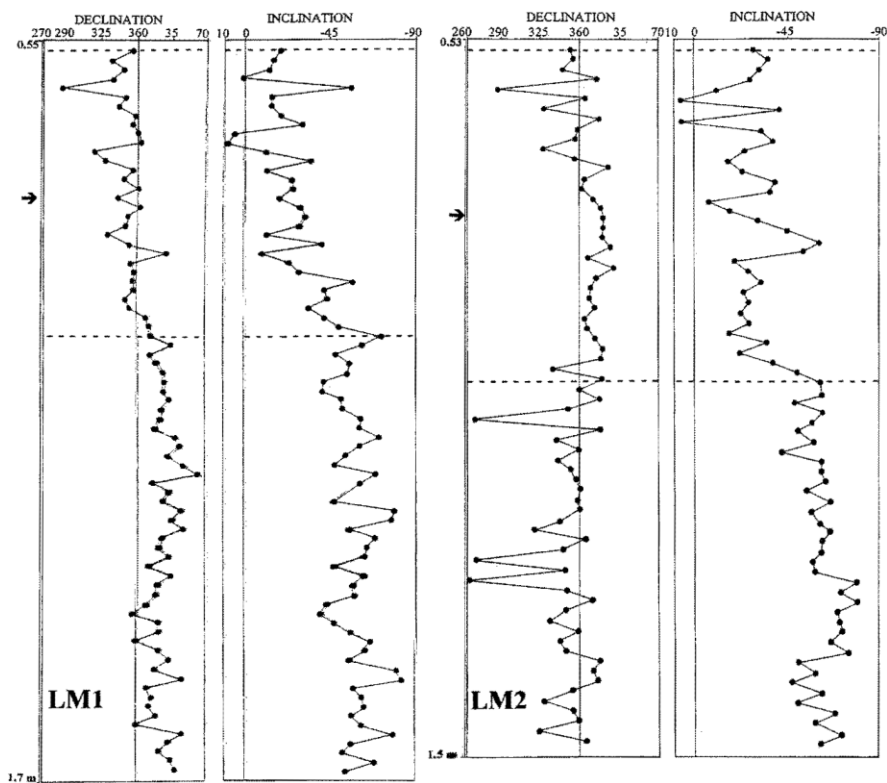
Figure 7. Stratigraphic presentation of the Declination and Inclination profiles from LM1 and LM2. The more conspicuous long directions departures are depicted between dashed lines.
