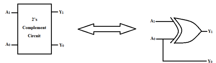
Fig 1: Block diagram and logic implementation of Complement Circuit using conventional approach
