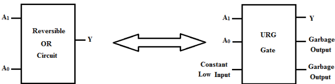
Fig 15: Block diagram and logic implementation of Reversible OR Circuit
