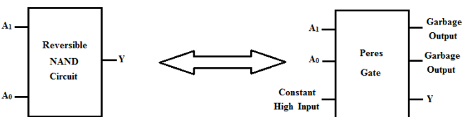
Fig 17: Block diagram and logic implementation of Reversible NAND Circuit
