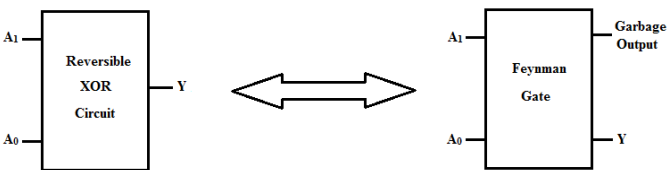
Fig 16: Block diagram and logic implementation of Reversible XOR Circuit
