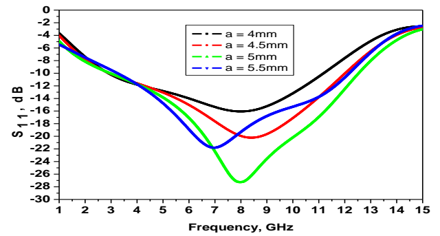
Fig. 4. S_{11} variation vs frequency for different values of the radius
