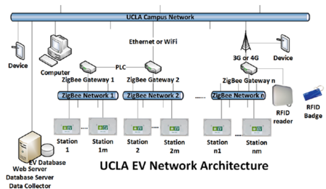
Figure 3. WINSmartEV™ Architecture
