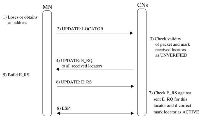
Fig. 2. Return routability tests and locator state.
