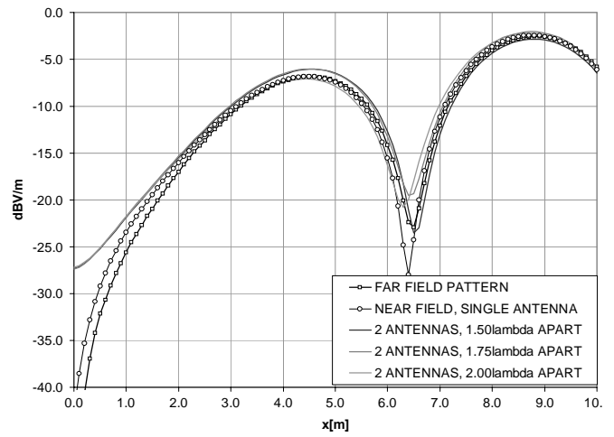
Fig. 12. Calculated electric field, \varphi = 0^\circ, z = -10\text{m}
