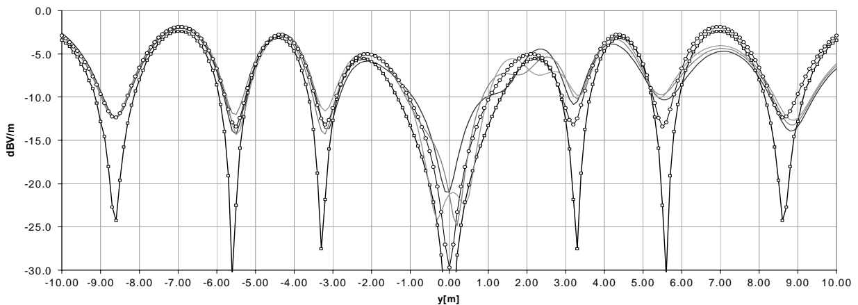
Fig. 14. Calculated electric field, \varphi = -90^\circ, +90^\circ, z = -5\text{ m} (legend from Fig. 13. applies)
