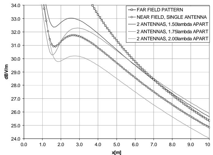
Fig. 10. Calculated electric field in the mainlobe direction, \varphi = 0^\circ , z = 0 \text{ m}
