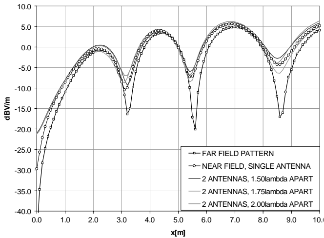
Fig. 11. Calculated electric field, \varphi = 0^\circ, z = -5\text{m}
