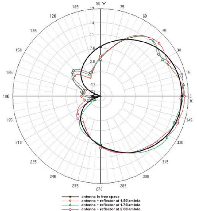
Fig. 6. Antenna in free space vs. Antenna + reflector, similar but slightly less distortion than for the previous configuration
