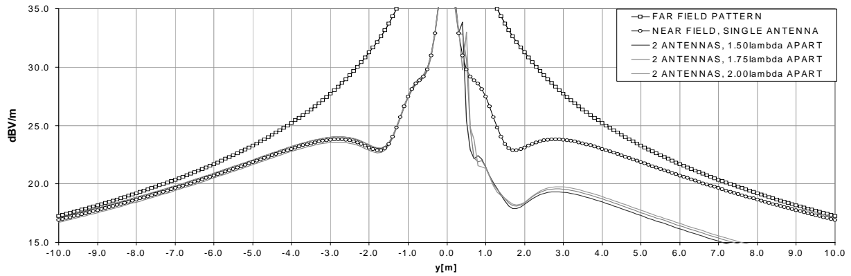
Fig. 13. Calculated electric field, \varphi = -90^\circ, +90^\circ, z = 0\text{ m}
