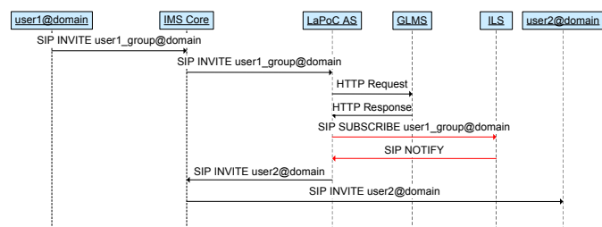
Fig. 5. Simplified LaPoC session establishment with groupInRange filters.
