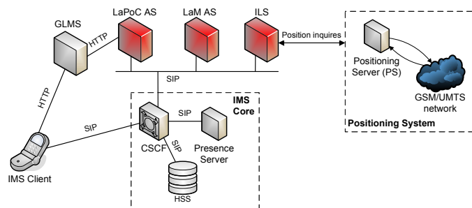
Fig. 2. Integration of the ILS in the IMS architecture.
