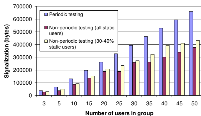
Fig. 9. Traffic load between ILS and MPS.
