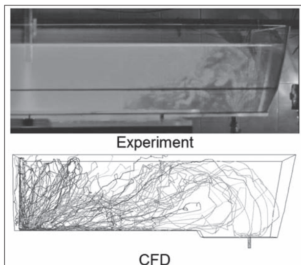
Figure 7 Particle distribution visualization obtained for water model and CFD model
