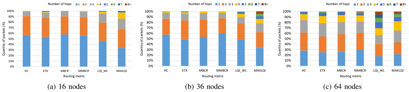
Fig. 7: Number of hops in the MP2P scenario.
