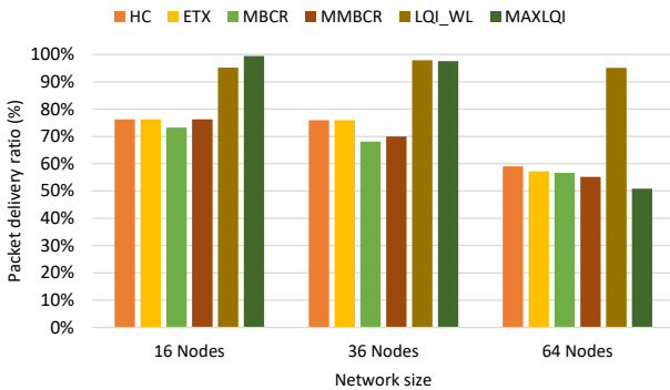
Fig. 8: Packet delivery ratio in the P2P scenario.
