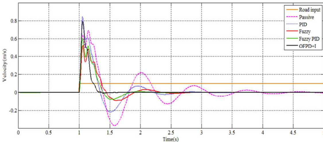
Fig. 15 Changes in the vehicle body velocity due to impact (road input of type I)
