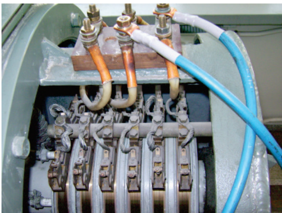
Figure 3 Commutator of healthy DC motor
