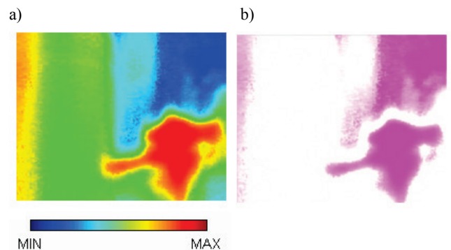
Figure 5 a) Thermographic image of commutator of shorted DC motor, b) Magenta color of thermographic image of commutator of shorted DC motor
