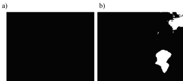
Figure 6 a) Magenta color of thermographic image of commutator of healthy DC motor after binarization for T = 0.1 , b) Magenta color of thermographic image of commutator of shorted DC motor after binarization for T = 0.1
