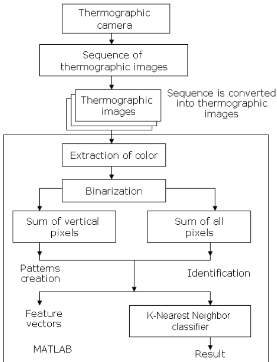
Figure 2 Fault diagnostic method of thermographic images of DC motor using extraction of color, binarization, sum of vertical pixels, sum of all pixels, K-Nearest Neighbor classifier
