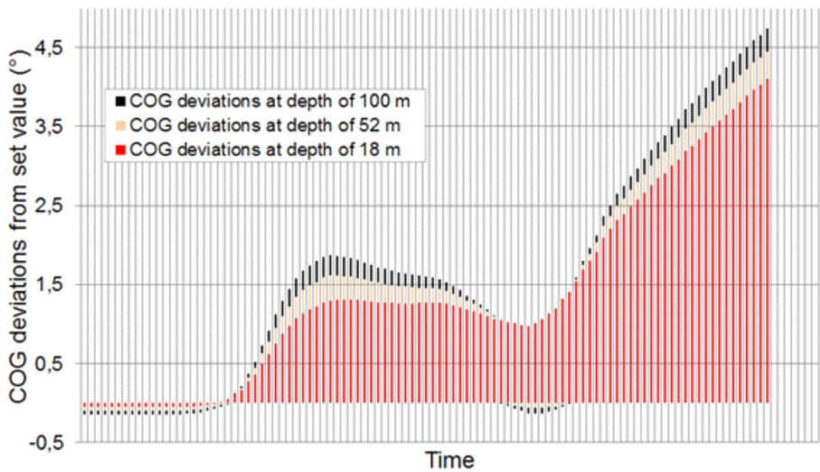
Figure 11: COG values changes regarding to set value of 180° for 100, 52 and 18 m of depth. Made by authors.
