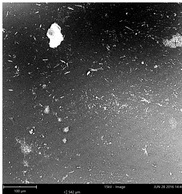
Figure 5. Scanning electron micrograph of conversion coated aluminum with a top coating of lacquer after immersion in 1 M NaCl solution for 170 h at 30 °C after application of adhesion tests.
