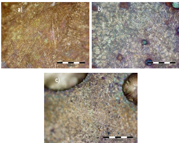
Figure 6 Optical micrographs of the CuAlNi alloy surfaces after the potentiodynamic polarization in the 0.1% a), 0.9% b) and 1.5% NaCl solution c)
