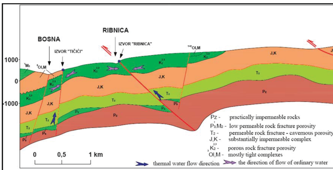
Figure 7: Hydrogeological profile of thermal water at Tičići and Ribnica near Kakanj Sc: H/V 1:100 000 (Šarić, 2015)
