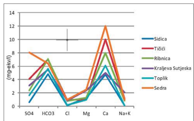
Figure 16: Schoeller diagram of thermal waters from the north-east periphery of Zenica-Sarajevo Basin (Šarić, 2015)
