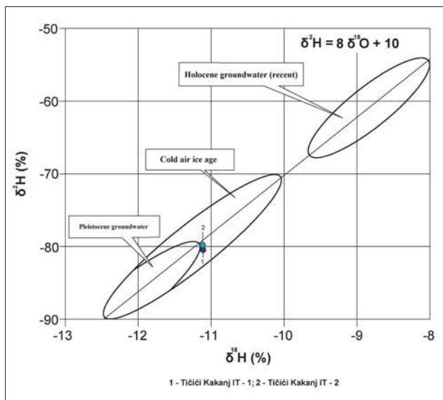
Figure 12: The correlation between δ 18 O and δ 2 H of thermal waters in Tičići (Šarić, 2015)
