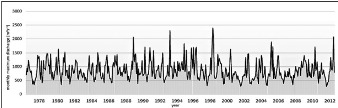
Fig. 5 Monthly precipitation at Varaždin and monthly maximum discharges of the Drava River at Botovo (data source: Meteorological and Hydrological Service of Croatia, DHMZ)
