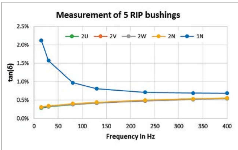
Figure 2. Dielectric loss measurement performed on 123 kV RIP bushings
