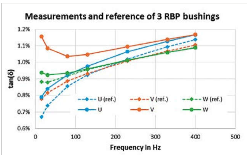
Figure 3. Dielectric measurements and reference measurements of three RBP bushings
