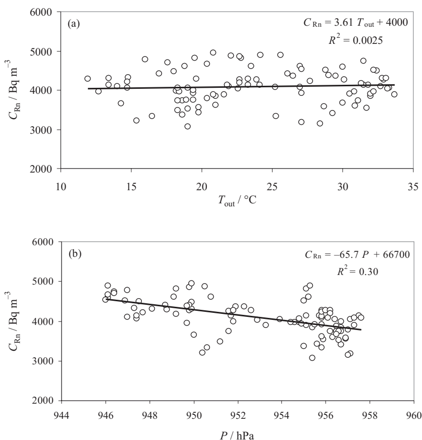
Figure 2. The dependence of radon concentration ( C_{Rn} ) on: (a) outdoor air temperature ( T_{out} ) and (b) barometric pressure ( P ) at the lowest point in the Postojna Cave, August 10–18, 1998.
