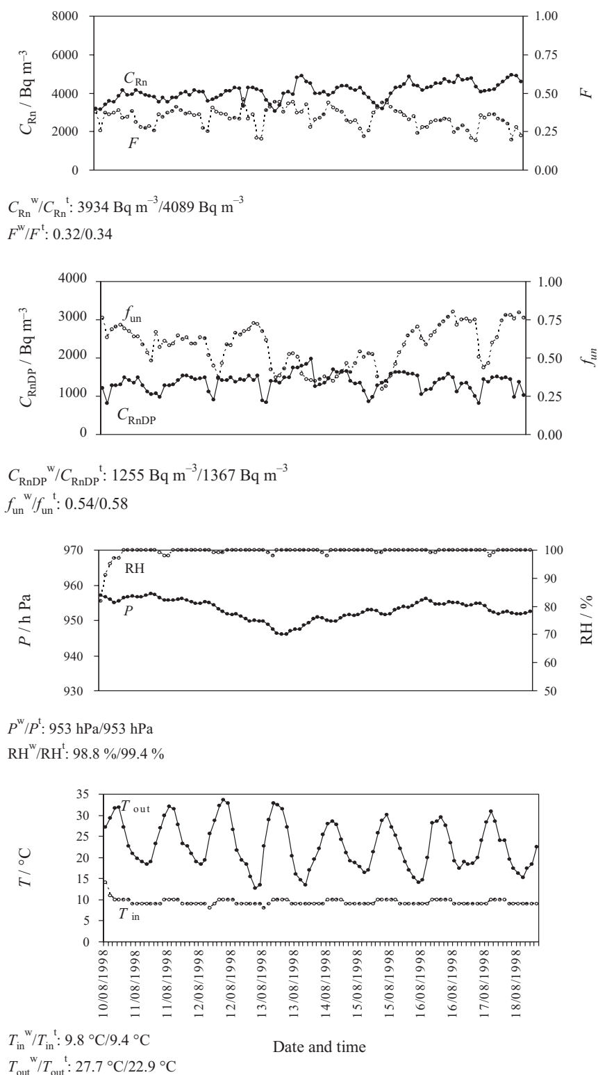
Figure 1. The lowest point in Postojna Cave, August 10–18, 1998: concentrations of radon ( C_{Rn} ) and radon decay products ( C_{RnDP} ), equilibrium factor ( F ), unattached fraction of radon decay products ( f_{un} ), barometric pressure ( P ), relative air humidity in the cave ( RH ), and air temperature in the cave ( T_{in} ) and outdoors ( T_{out} ). Average values during the whole period of measurement (denoted by t – total) and during the working hours only (denoted by w – working) are quoted for each parameter.
