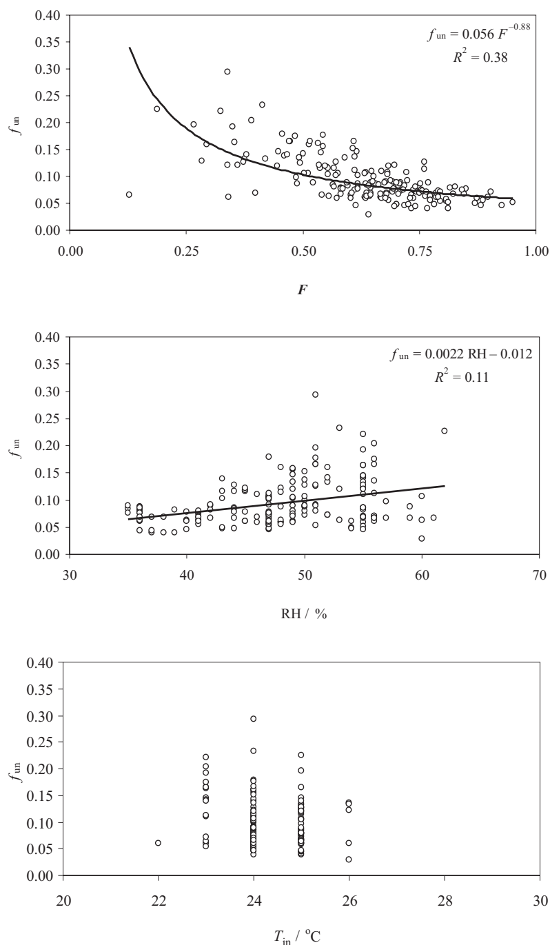
Figure 5. Dependence of the unattached fraction of RnDP ( f_{un} ) on: (a) equilibrium factor ( F ), (b) relative humidity of indoor air (RH) and (c) indoor air temperature ( T_{in} ) in the kindergarten, from December 28, 2000 to January 11, 2001.
