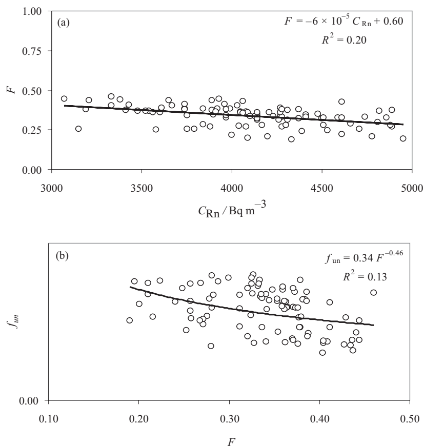
Figure 3. The dependence of: (a) equilibrium factor ( F ) on radon concentration ( C_{Rn} ) and (b) unattached fraction of RnDP ( f_{un} ) on the equilibrium factor ( F ) at the lowest point in the Postojna Cave, August 10–18, 1998.
