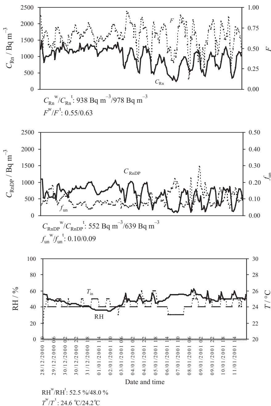
Figure 4. The kindergarten, from December 28, 2000 to January 11, 2001: concentrations of radon ( C_{Rn} ) and radon decay products ( C_{RnDP} ), equilibrium factor ( F ), unattached fraction of radon decay products ( f_{un} ), relative air humidity in the cave (RH), and air temperature ( T_{in} ). Average values during the whole period of measurement (denoted by t – total) and during the working hours only (denoted by w – working) are quoted for each parameter.
